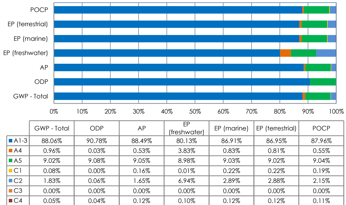
Figure 1 - shows the relative contribution of each life cycle stage to different environmental indicators for the carbon steel reinforcing bar products manufactured by the primary (BF-BOF) production route
